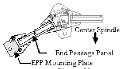
Figure 22 Install Mounting Plate
