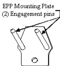
Figure 21 Identify End Mounting Plate
