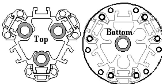
Figure 45 Identify Center Column
